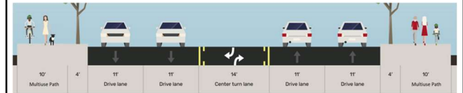
Segment 2: 2 Lanes, TWLTL, 10' Mixed-use path
