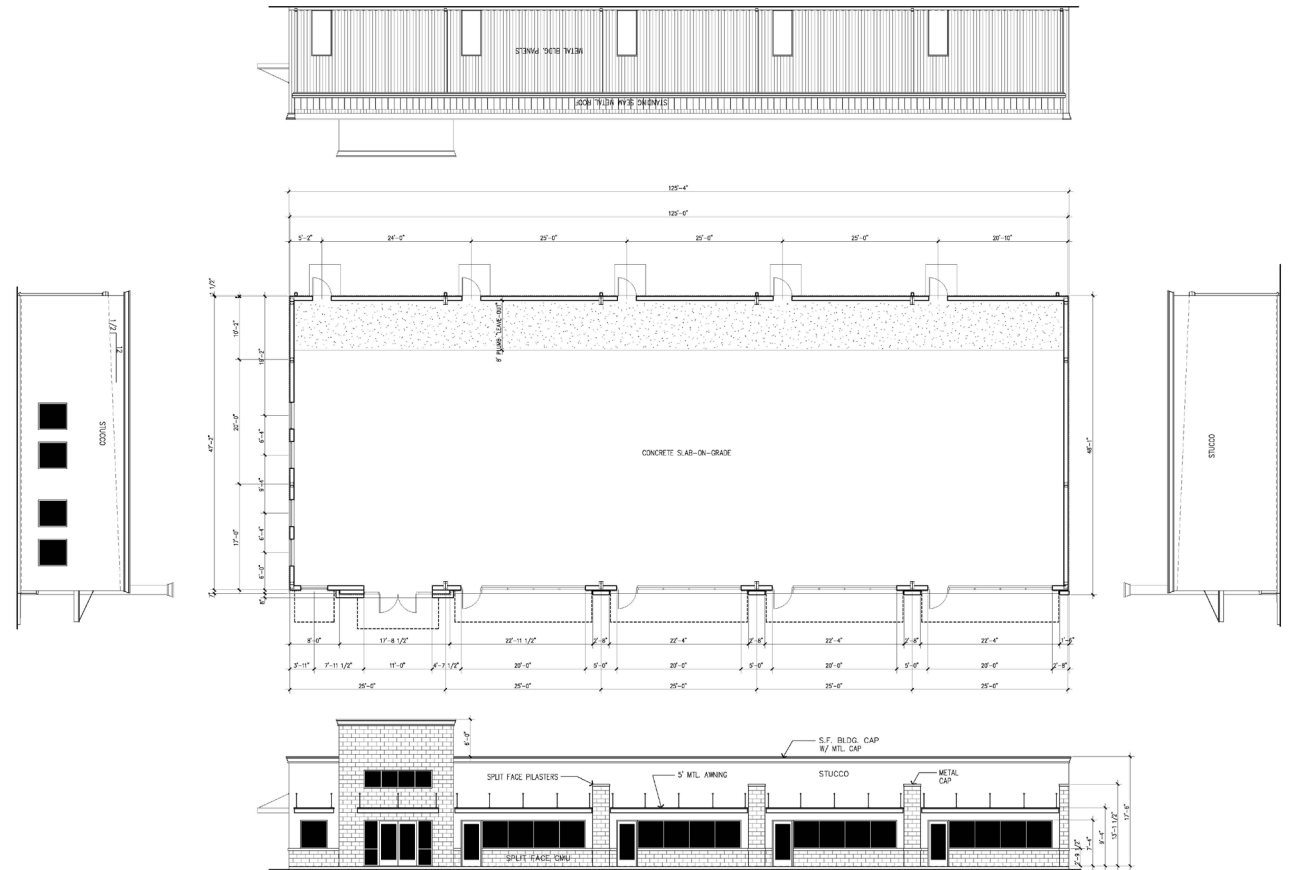
YEN RABE SCHEMATIC FLOOR PLAN & ELEVATIONS 03.07.16 WYCOFF DEVELOPMENT AND CONSTRUCTION L.L.C. 1/8" = 1'-0"
